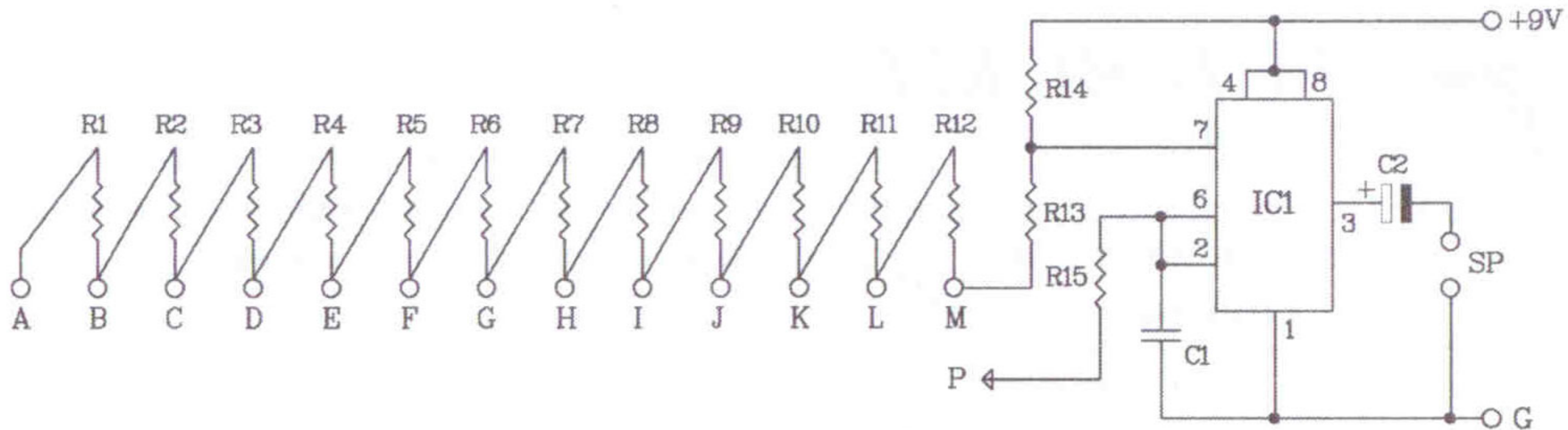
Figure 2. The mini organ 13 tone circuit
