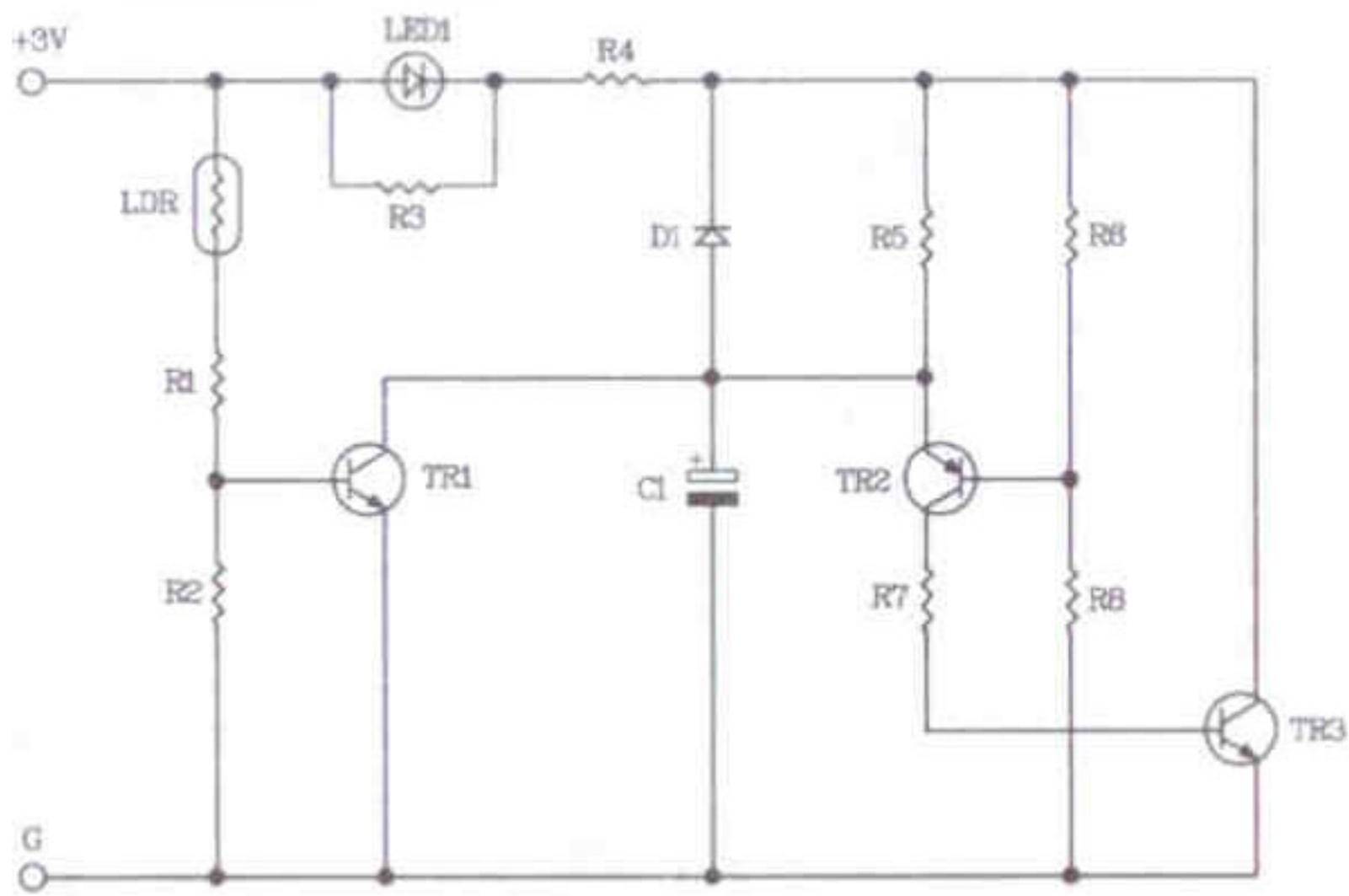
Figure 2. The firefly light (night activate) circuit
